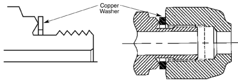
Figure 75: BSPP
